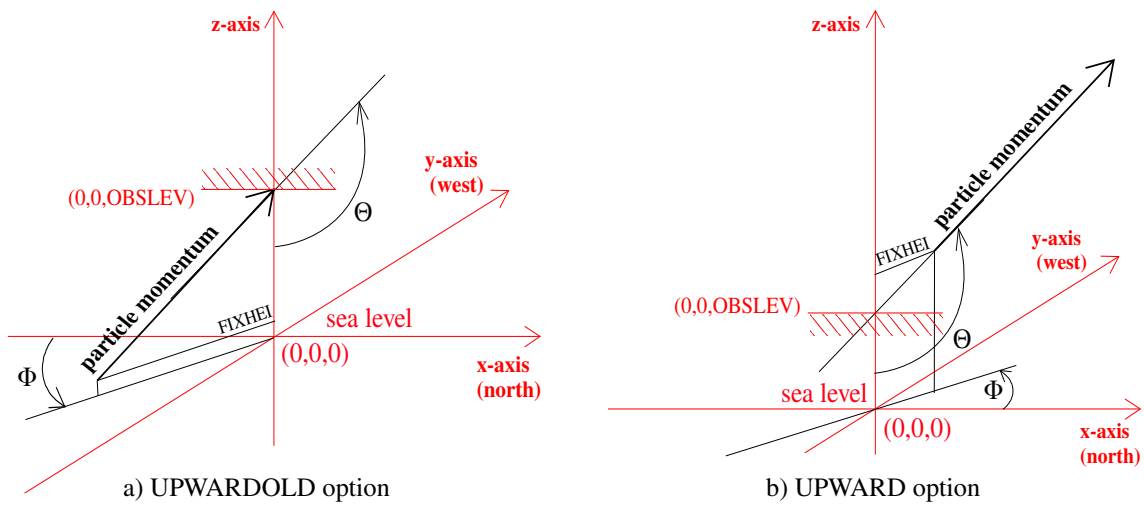
Figure 2: Coordinate system in CORSIKA for upward going showers.
